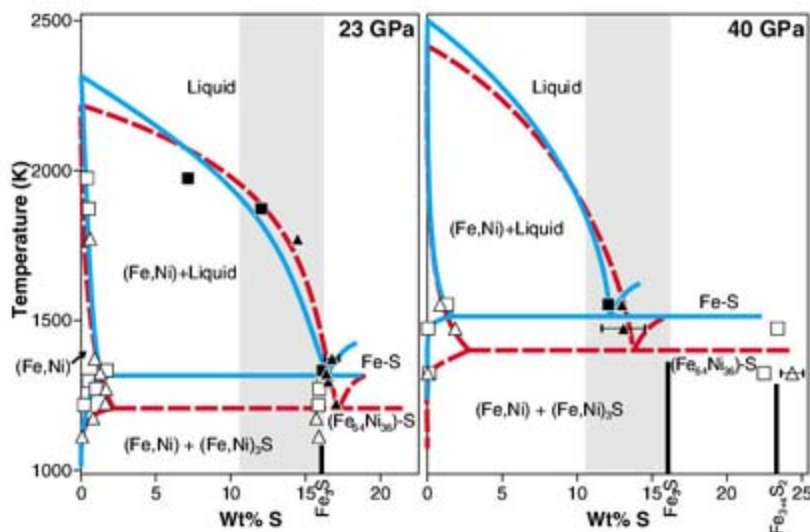
Fig. 1. Fe-S and (Fe,Ni)-S phase diagrams at 23 (left) and 40 (right) GPa. Fe-S results, squares; (Fe,Ni)-S results, triangles; liquid phases, black symbols; solids, white symbols. The resulting phase boundaries for Fe-S (solid blue lines) and (Fe,Ni)-S (dashed red lines) are shown. Thick black vertical lines indicate the composition of stable sulfide phases, as indicated along the x axis. Temperatures for melting of pure Fe are from Boehler (20). Pure Fe-Ni melting temperatures at both pressures are based on the melting depression from pure Fe of roughly 80 K observed at 1 atm for \text{Fe}_{64}\text{Ni}_{36} . The gray shaded region represents the estimated bulk martian core composition (1–3). Error bars ( 1\sigma ) represent analytical variation and are indicated when larger than the symbol.
